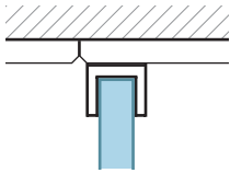
Wandprofil AP Profil mural apparent
